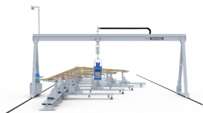
PORTAL GANTRY
